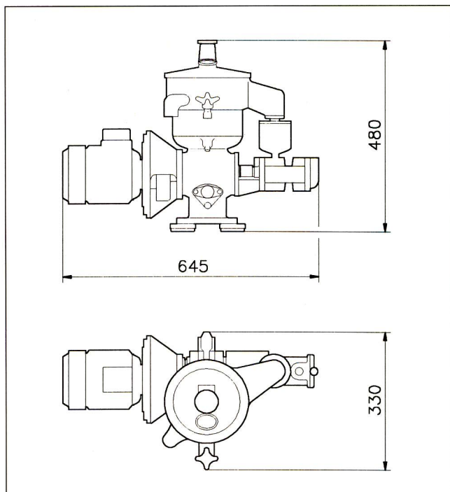
Fig.3 Dimension drawing
